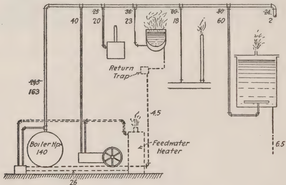
FIG. 11 IMPROVED STEAM DISTRIBUTION
